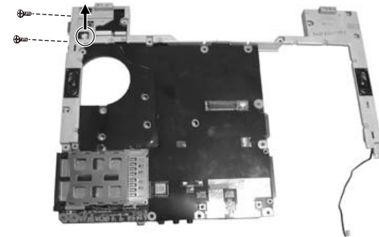
Figure 2-31 Free the system board
