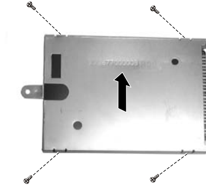
Figure 2-9 Remove hard disk drive
